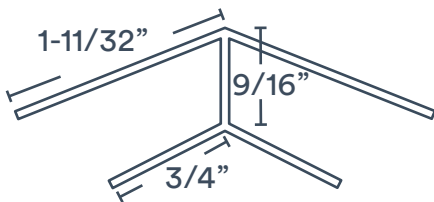
45° H Channel
